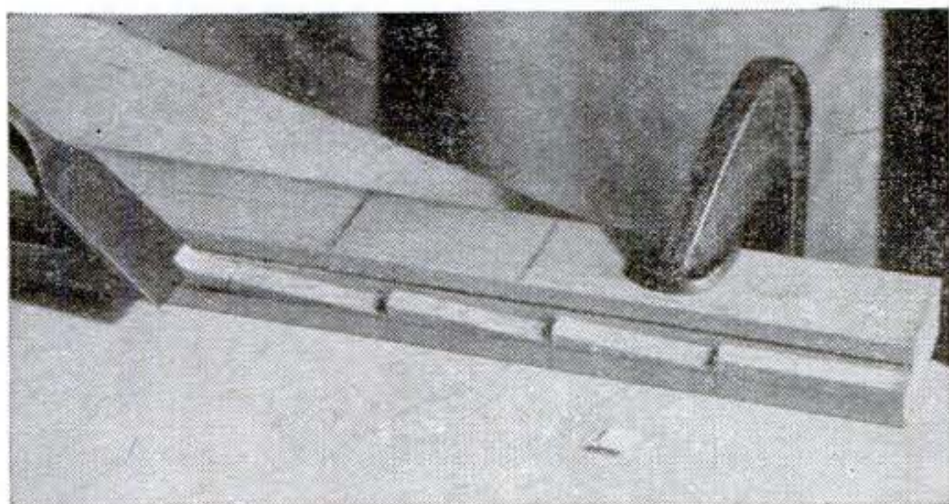
Chisel out each notch after cutting kerfs as shown in the drawing. Space them 1 7/8" apart.
